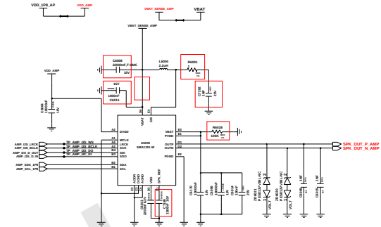
Audio amp
